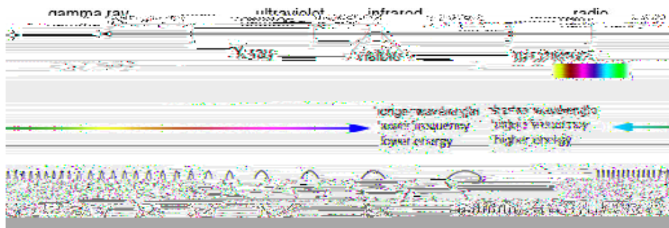
Electromagnetic Spectrum.
